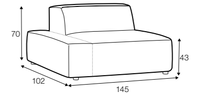
bench 145x102 left or right
